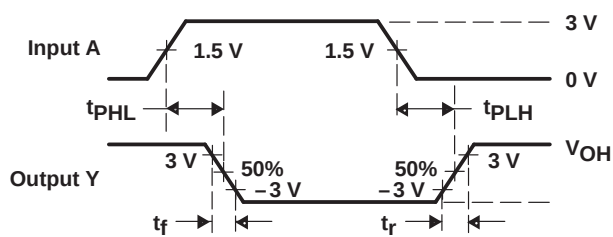
DRIVER VOLTAGE WAVEFORMS (see Note C)
