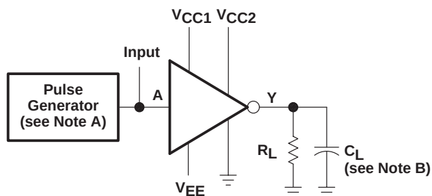
DRIVER TEST CIRCUIT
